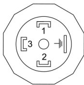
Solenoid plug
